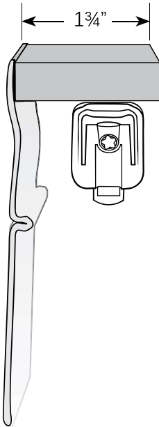
MANUAL CORDLESS HEAD RAIL
