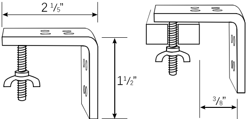
CLUTCH BRACKET/ MOTORIZED CORDLESS BRACKET
