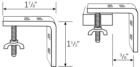
MANUAL CORDLESS BRACKET
