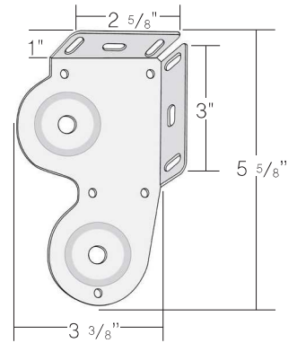
DUAL BRACKET
